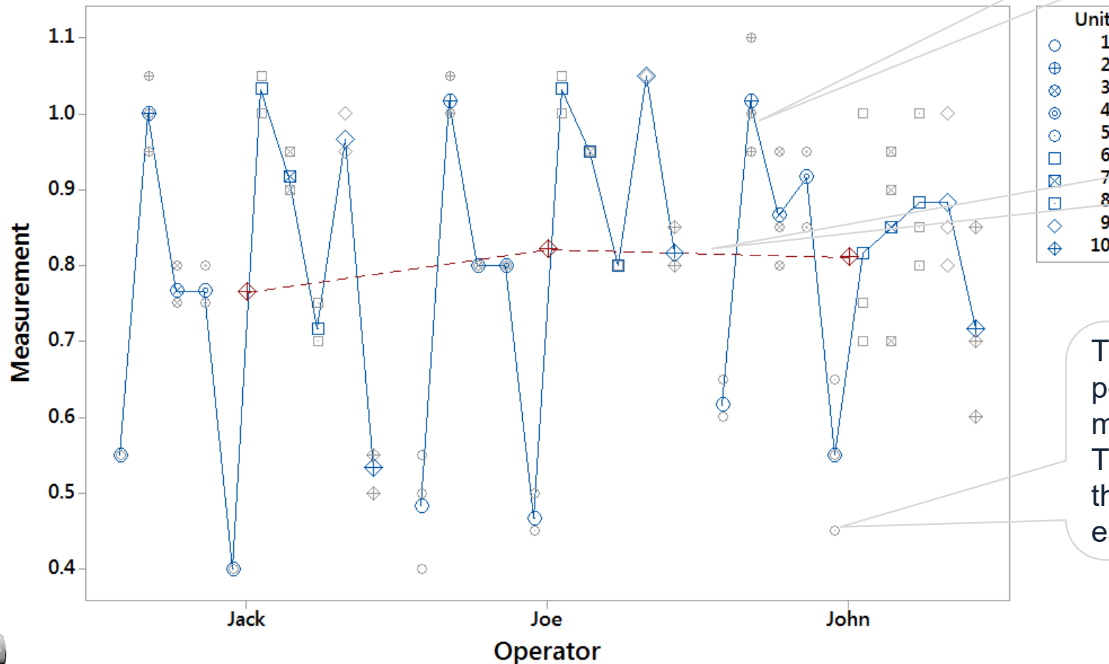
Multi-Vari Chart for Measurement by Unit - Operator
